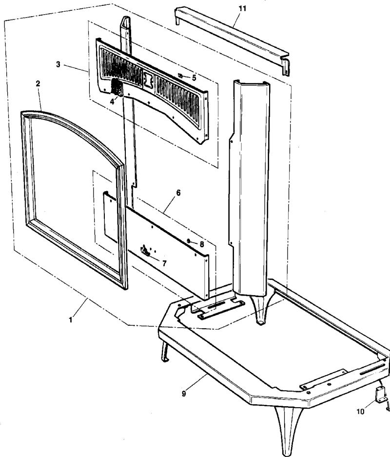
902FKL Traditional Fascia & Base with Legs
