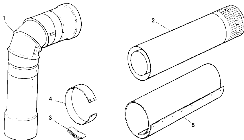
903VKT Vent Unit
