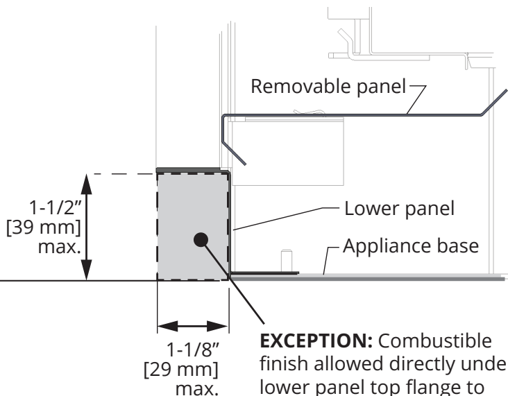
Right side view of appliance - bottom
