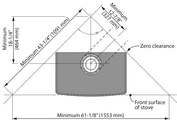
Corner clearances
