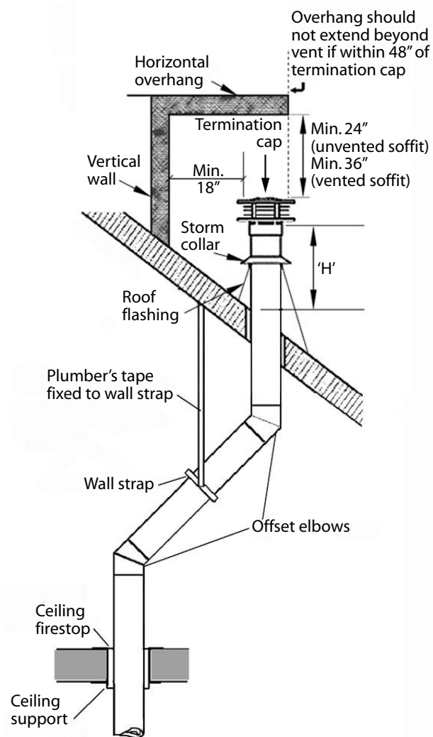
Through-the-roof installation
