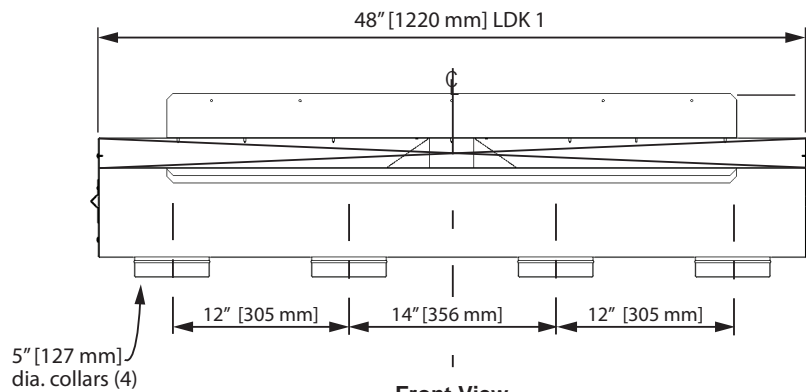
Front View
