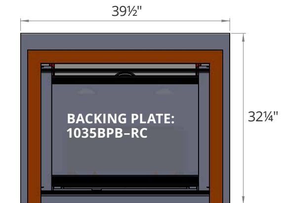
3-SIDED Backing plate sits flush with bottom of appliance.
