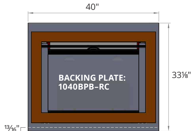
4-SIDED Backing Plate overhangs bottom of appliance.
