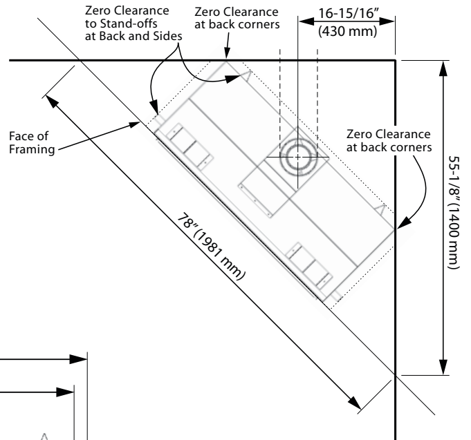
Corner Dimensions
